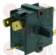
1057036 SELECTOR SWITCH 0-3 POSITIONS 10A 250V D-shaped pin 6x4.6 mm
